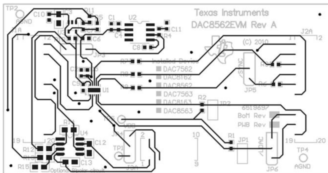
Figure 3. DAC8562EVM: Top Layer Image
