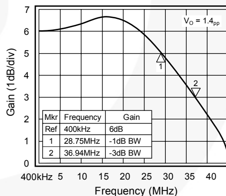
Figure 8. Bypass Mode Frequency Response
