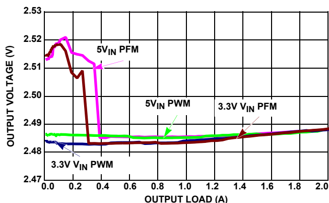
FIGURE 10. V_{OUT} REGULATION vs LOAD, 2.25MHz, 2.5V CHANNEL1
