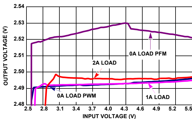
FIGURE 12. OUTPUT VOLTAGE REGULATION vs V_{IN} 2.5V CHANNEL 1
