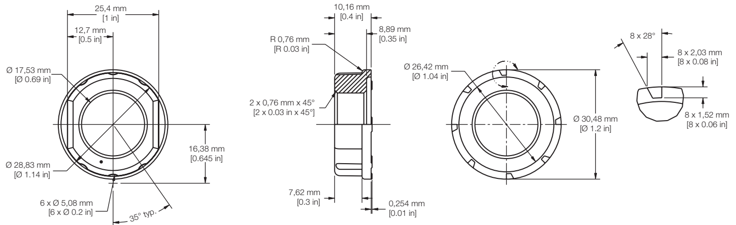
Figure 14. Mounting clip 87770
