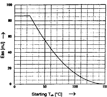
Avalanche Energy Derating
