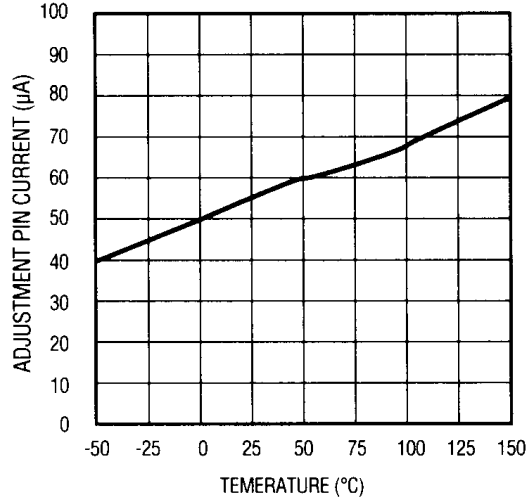
TEMPERATURE STABILITY
