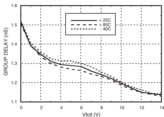
Group Delay vs. Fcenter vs. Temperature
