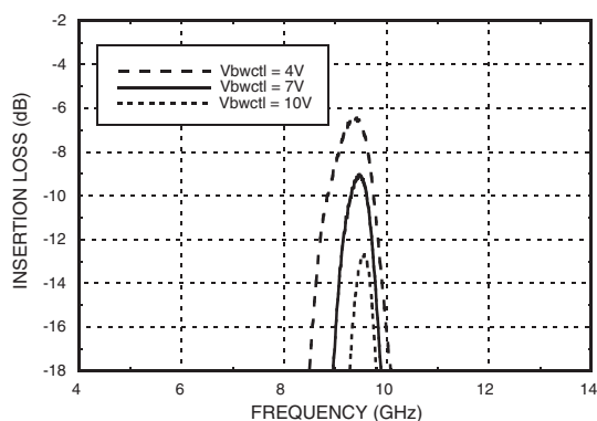
Insertion Loss vs. Vbwctl, Vfctl = 7V
