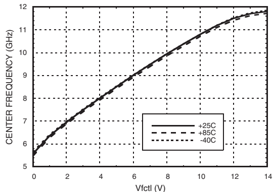
Center Frequency vs. Temperature, Vfctl = Vbwctl
