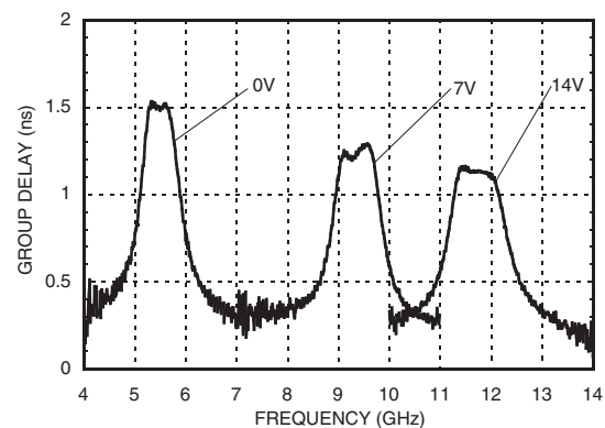
Group Delay, V_{ctl} = V_{bwctl}
