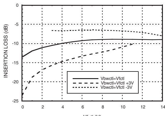
Insertion Loss vs. Bandwidth Control
