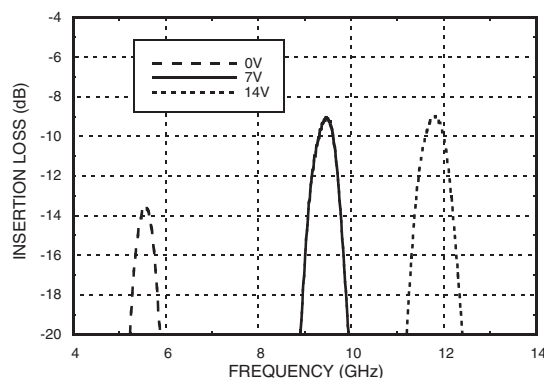
Insertion Loss vs. Control Voltages, V_{fctl} = V_{bwctl}
