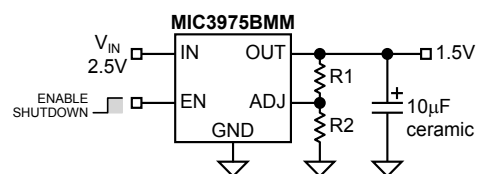
1.5V/750mA Adjustable Regulator
