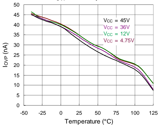
I_{OVP} vs. Temperature
