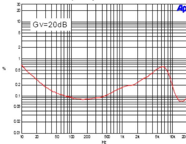
9. THD Frequency—BTL
