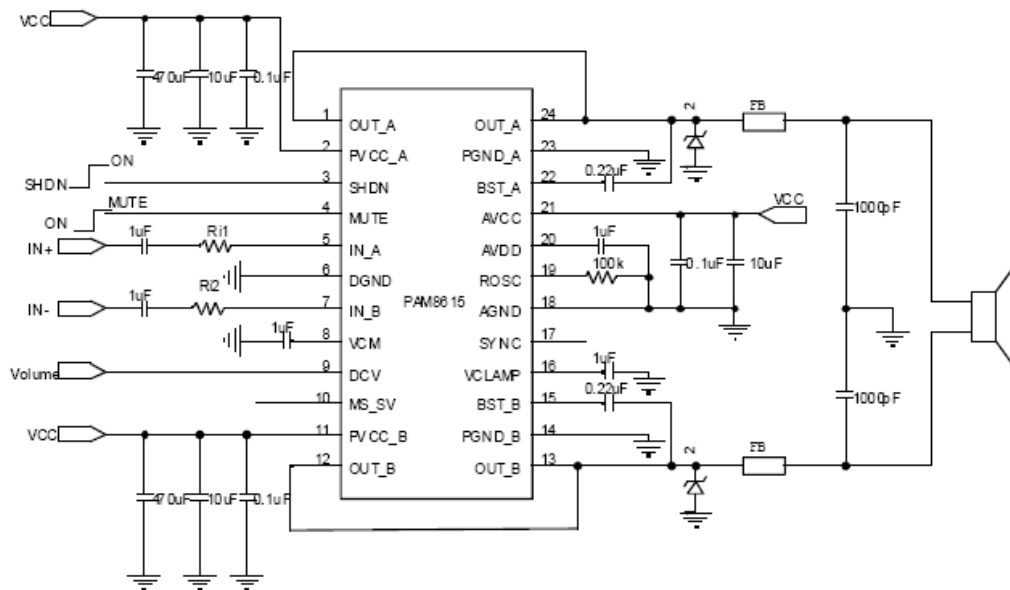
BTL Configuration
