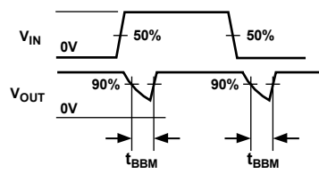
Figure 19. Break-Before-Make Time Delay, t_{BBM} (ADG619 Only)
