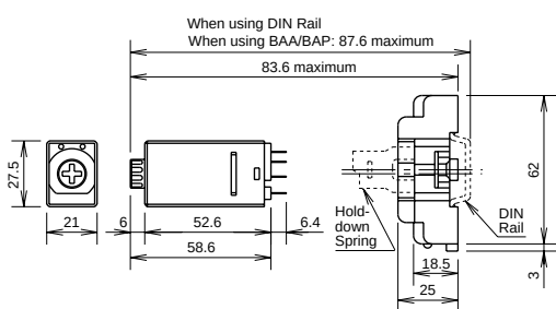
GT5Y Timer, Blade with SY4S-05
