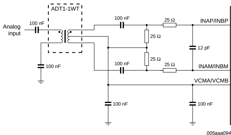
Fig 18. Single transformer configuration suitable for baseband applications
