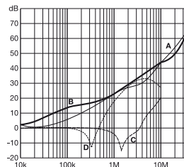
FN 9233: 6 to 10A types
