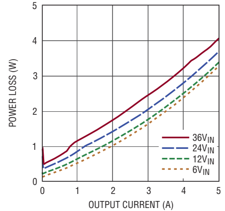
Power Loss vs Output Current, 1.2V_{OUT}
