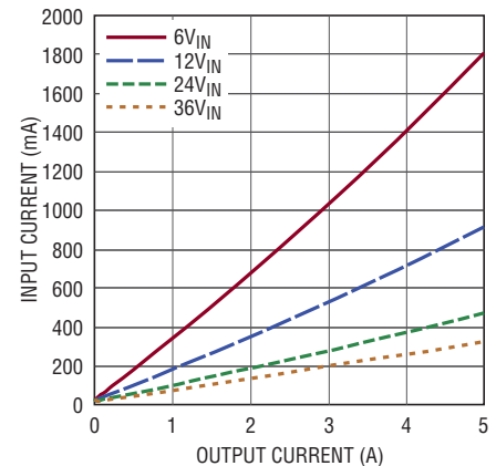
Input Current vs Output Current, 1.5V_{OUT}
