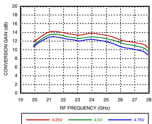
Conversion Gain, LSB vs. Vdd
