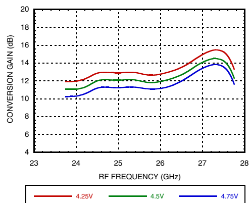
Conversion Gain, USB vs. Vdd
