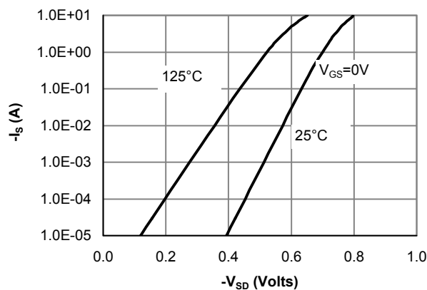
Figure 6: Body-Diode Characteristics
