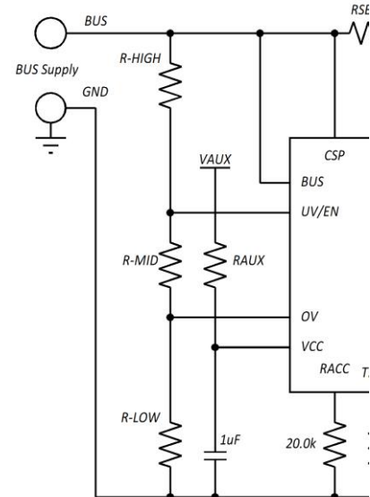
Figure 6 - External VAUX connection for lower BUS voltages.
