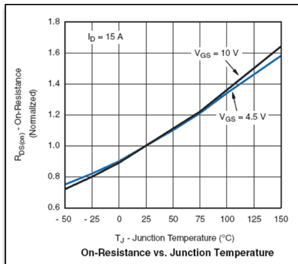
Figure 14 - Examples of an R_{DS(ON)} (left) and a R_{DS(SCALAR)} thermal scalar (right) graphs.
