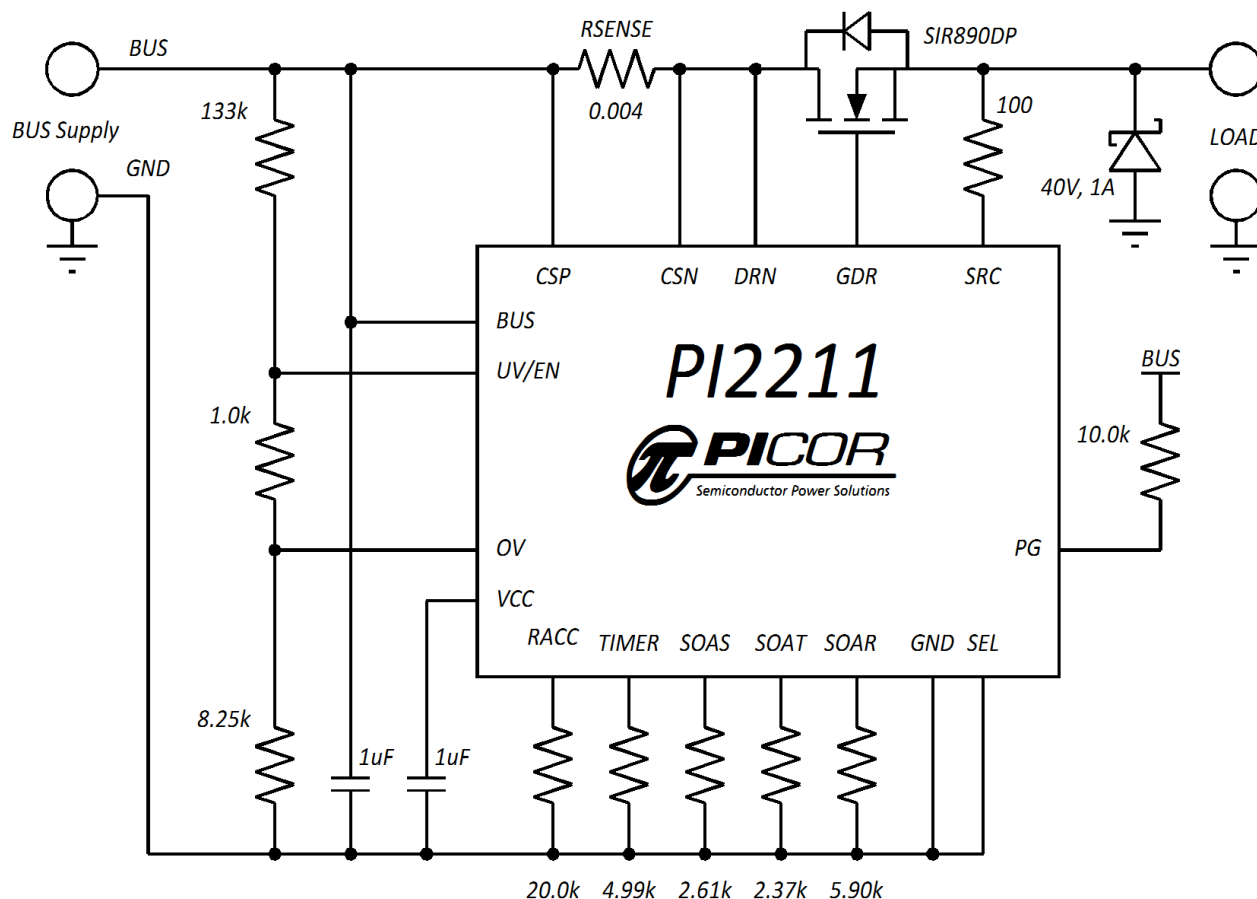
Figure 13 - Final Design Schematic
