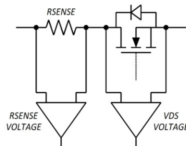
Figure 15 - MOSFET Power measurements.
