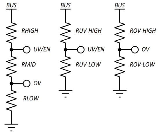
Figure 17 - Resistor divider options for UV and OV threshold programming.
