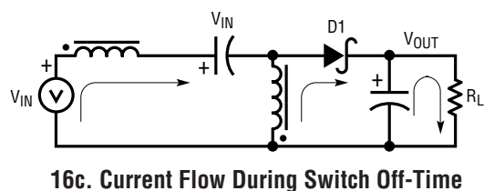
Figures 16. SEPIC Topology and Current Flow
