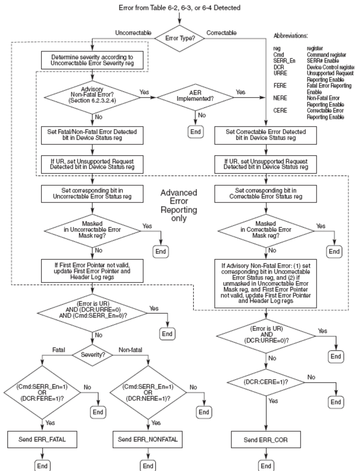
Figure 22: PCIe Flowchart of Device Error Signaling and Logging Operations
