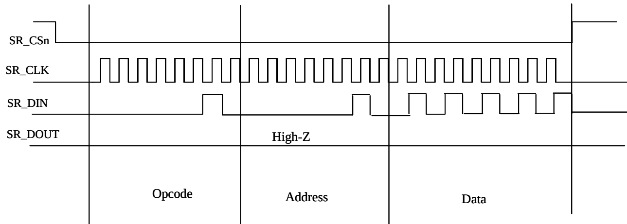
Figure 33: 9-bit EEPROM Write Timing
