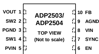
Figure 2. Pin Configuration
