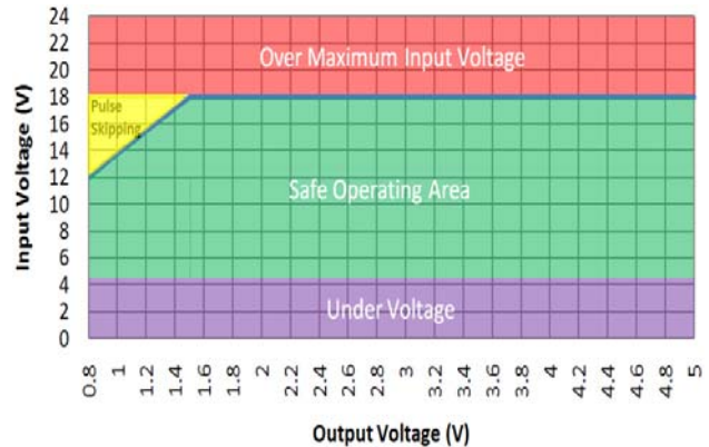
Figure 41. NCP3170A Safe Operating Area
