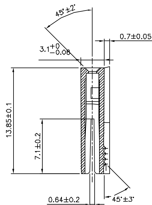
SECTION WW
