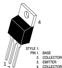
CASE 221A-06 TO-220AB
