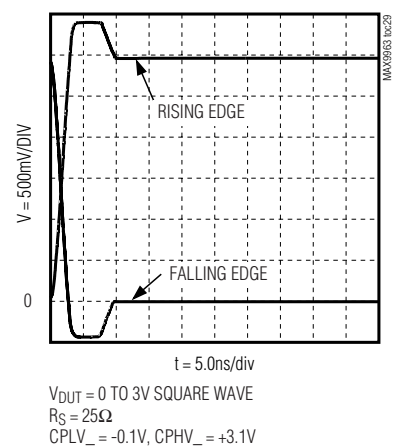
CLAMP RESPONSE
