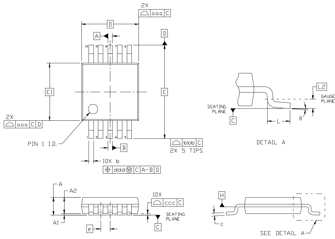
Figure 15. 10-pin MSOP Package Drawing
