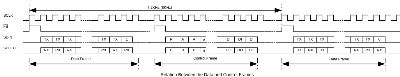
Figure 3: Serial Port Timing Diagram
