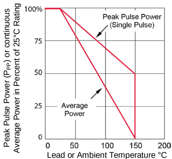
FIGURE 3 Derating Curve
