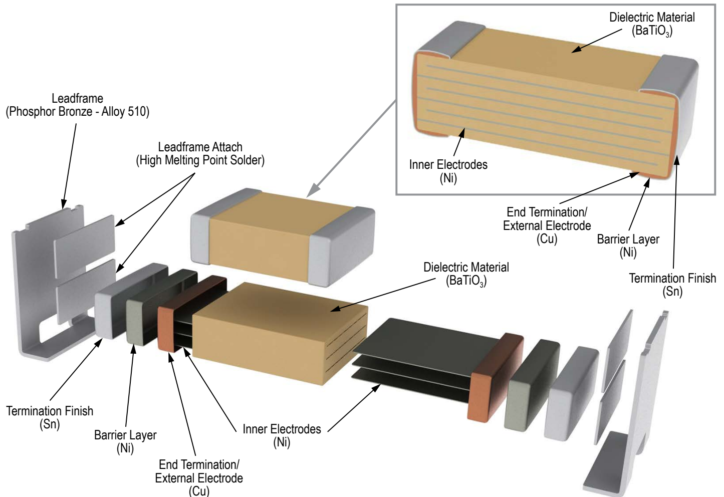
Detailed Cross Section
