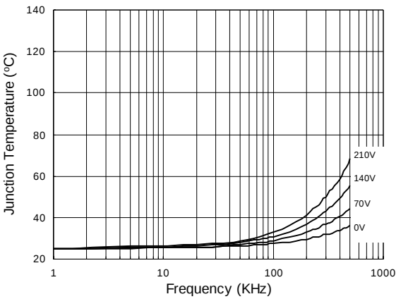
Figure 24. IR2106 vs Frequency (IRFBC20) R gate = 33Ω, V CC = 15V
