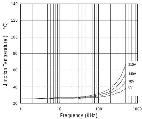
Figure 33. IR21064 vs Frequency (IRFBC30) R gate = 22Ω, V CC = 15V
