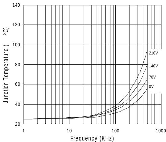
Figure 35. IR21064 vs Frequency (IRFPE50) R gate = 10Ω, V CC = 15V
