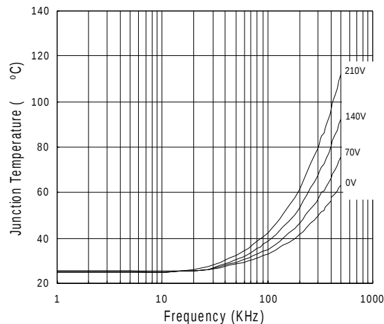
Figure 30. R2106S vs Frequency (IRFBC40) Rgate = 15Ω, VCC = 15V
