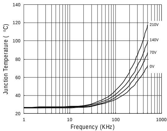
Figure 27. IR2106 vs Frequency (IRFPE50) R_{gate} = 10\Omega , V_{CC} = 15V
