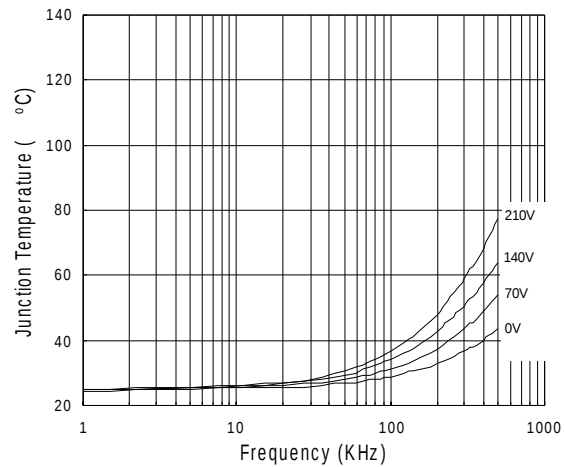
Figure 34. IR21064 vs Frequency (IRFBC40) R gate = 15Ω, V CC = 15V
