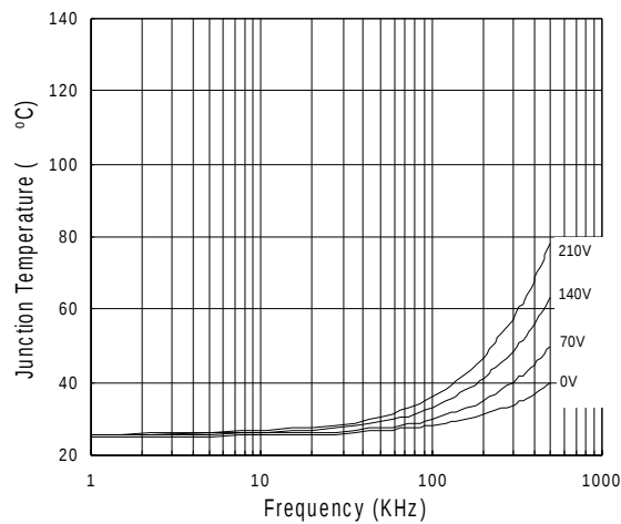
Figure 37. R21064S vs Frequency (IRFBC30) Rgate = 22Ω, VCC = 15V
