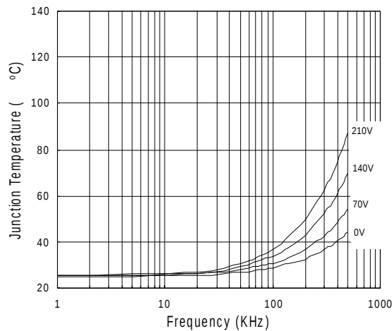
Figure 29. R2106 vs Frequency (IRFBC30) Rgate = 22Ω, VCC = 15V
