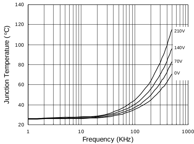
Figure 39. R21064S vs Frequency (IRFPE50) Rgate = 10Ω, VCC = 15V
