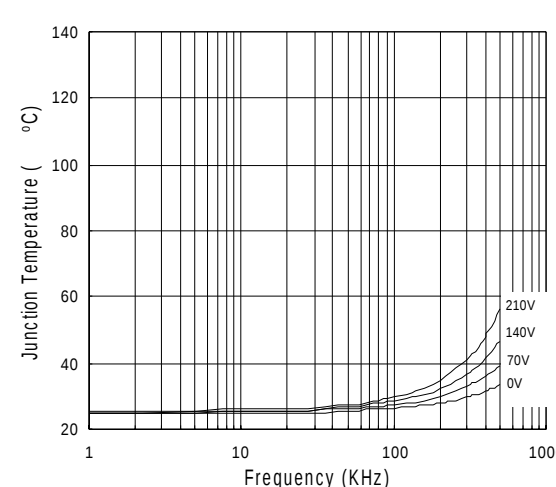
Figure 32. IR21064 vs Frequency (IRFBC20) Rgate = 33Ω, VCC = 15V
