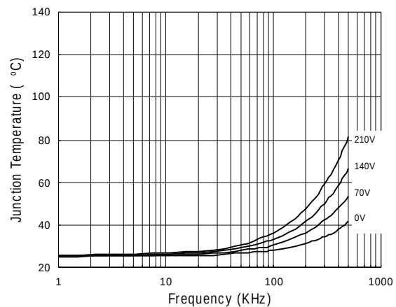
Figure 28. IR2106S vs Frequency (IRFBC20) R_{gate} = 33\Omega , V_{CC} = 15V
