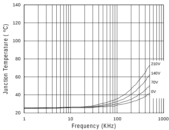
Figure 25. IR2106 vs Frequency (IRFBC30) R_{gate} = 22\Omega , V_{CC} = 15V
