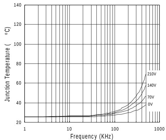
Figure 36. IR21064S vs Frequency (IRFBC20) R gate = 33Ω, V CC = 15V
