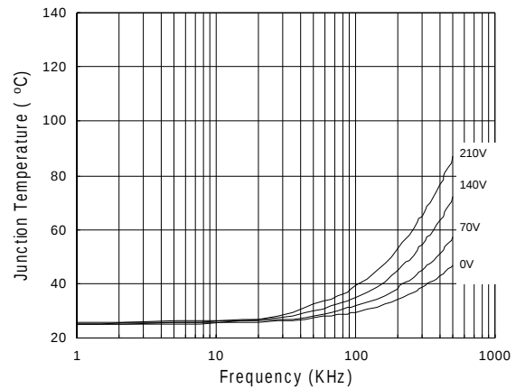
Figure 26. IR2106 vs Frequency (IRFBC40) R_{gate} = 15\Omega , V_{CC} = 15V
