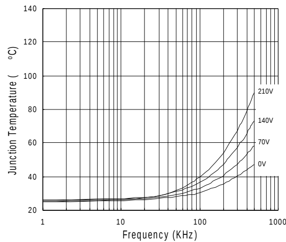
Figure 38. R21064S vs Frequency (IRFBC40) Rgate = 15Ω, VCC = 15V
