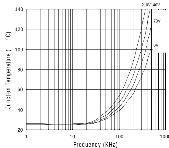
Figure 31. R2106S vs Frequency (IRFPE50) Rgate = 10Ω, VCC = 15V
