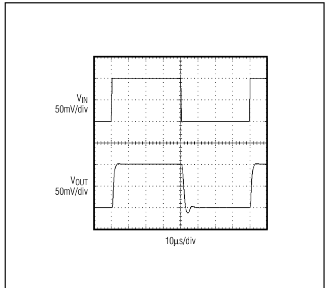
Figure 8b. Driving a 5000pF Capacitive Load with a 47 \Omega Isolation Resistor
