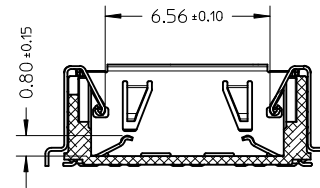
SECTION Y-Y
