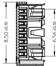
SECTION Z-Z
