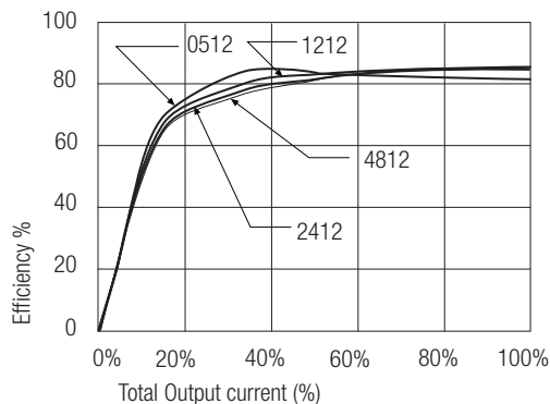
Efficiency / Load
