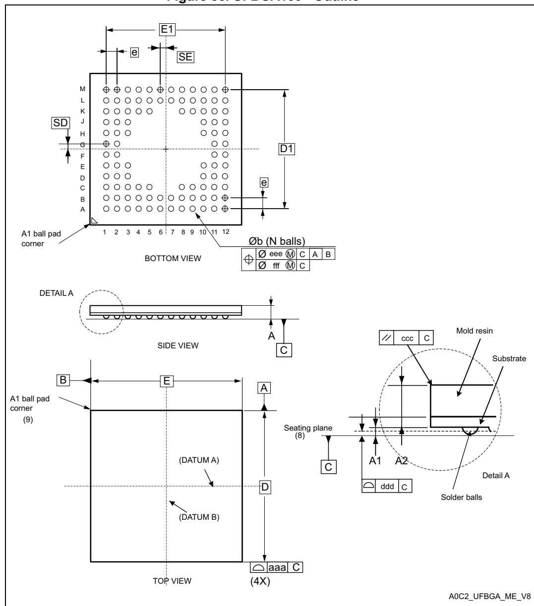
Figure 56. UFBGA100 - Outline (13)
