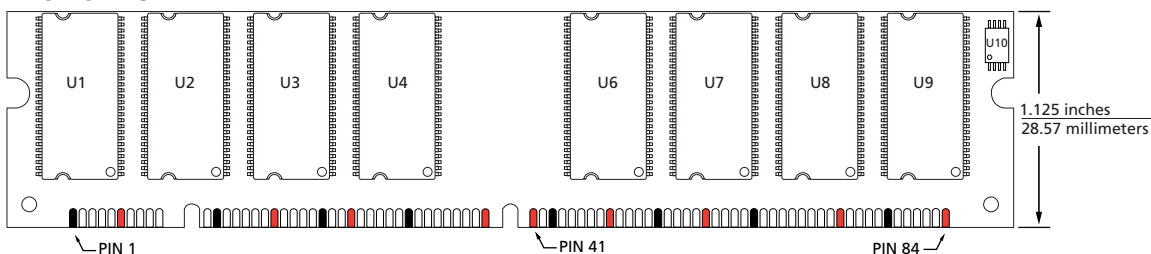
Figure 2: Pin Locations (168-Pin DIMM)
