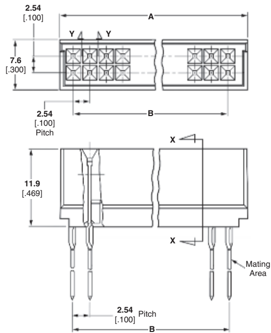
Section Y-Y
