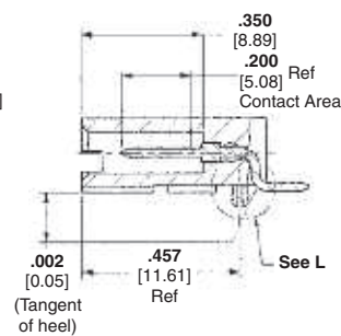
Section K-K
