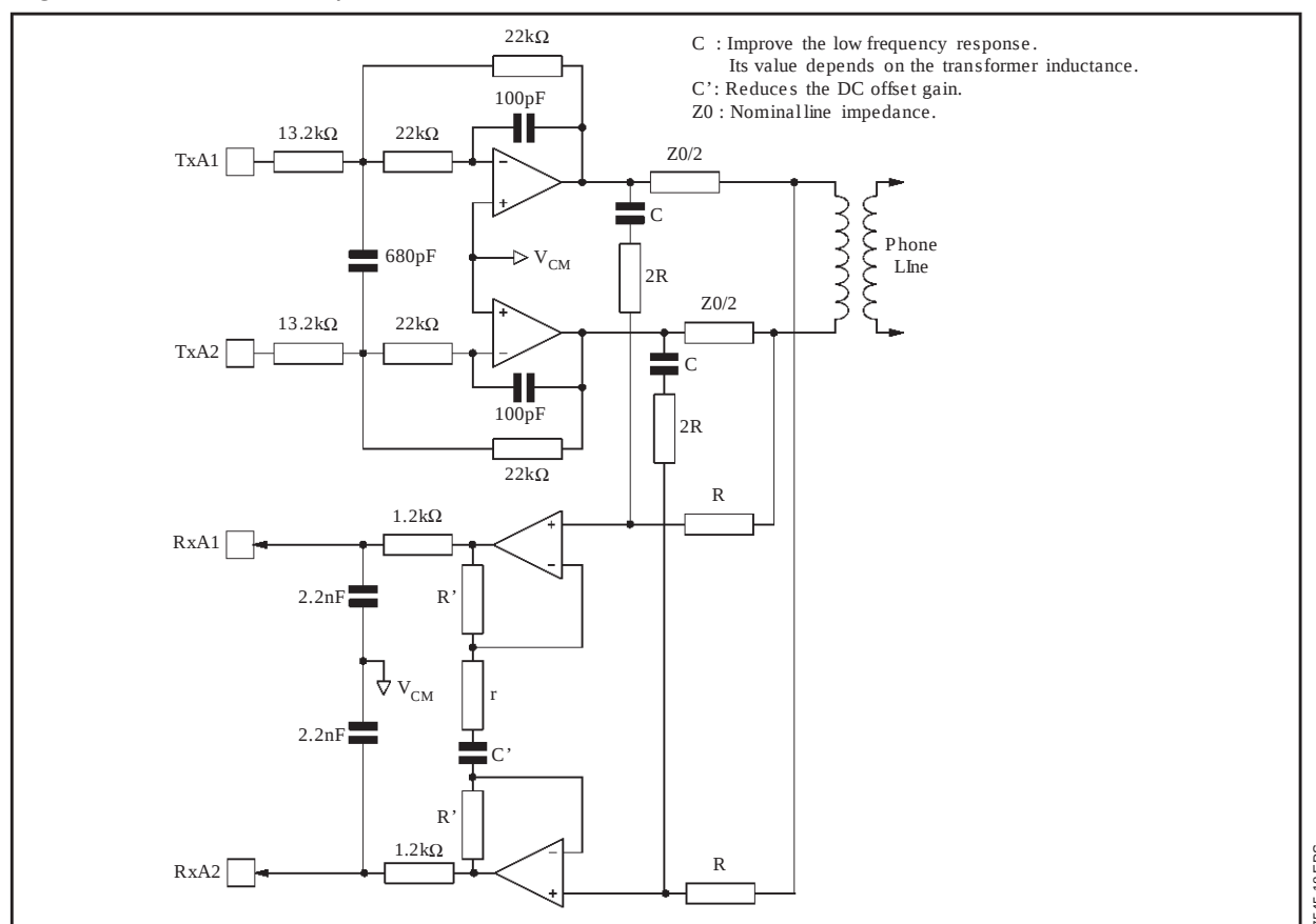
Figure 16 : Differential Duplexer
