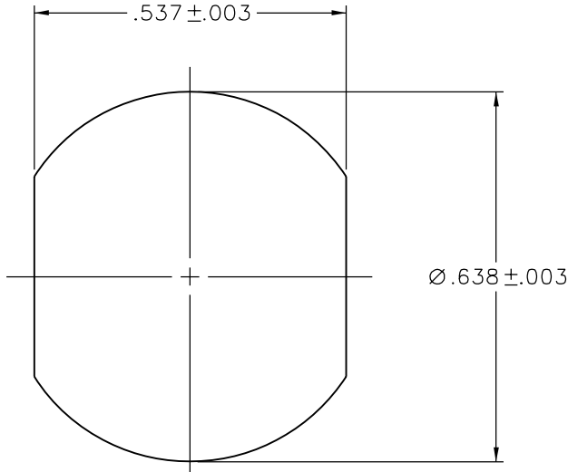
MOUNTING HOLE
