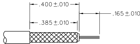
CABLE STRIP DIMENSIONS NOT TO SCALE
