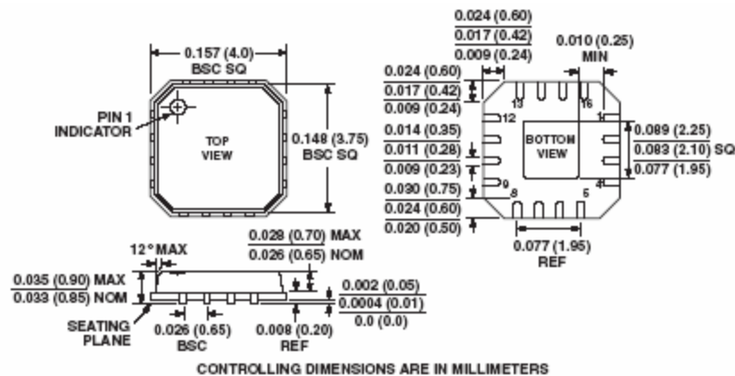
Figure 29. 16-Lead Lead Frame Chip Scale Package [LF CSP] 4mm × 4 mm (CP-16)
