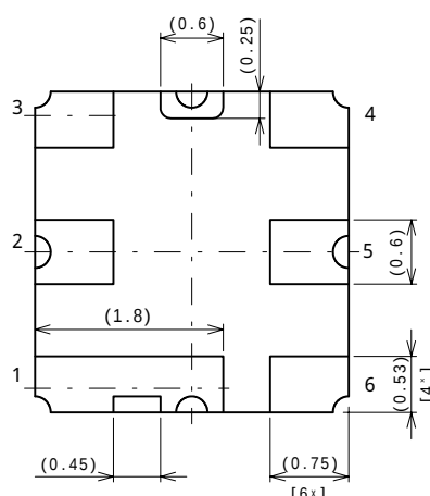
Fig.2 Package dimensions (in mm)
