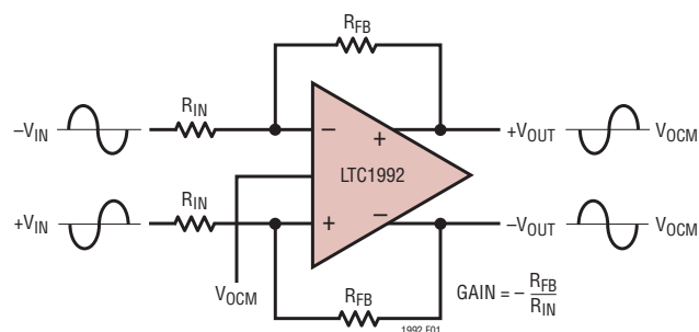
Figure 1. Comparison of an Op Amp and a Fully Differential Amplifier
