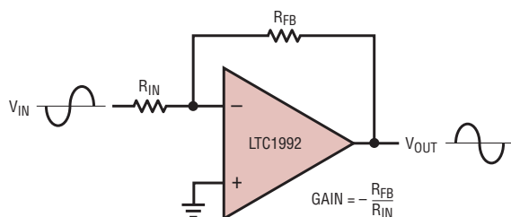
Figure 1. Comparison of an Op Amp and a Fully Differential Amplifier
