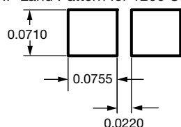
PHP Land Pattern for 1206 Case Size
