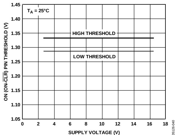
Figure 22. ON (ON-CLR) Pin Threshold vs. Supply Voltage
