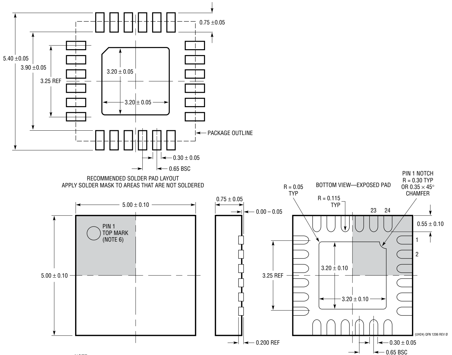
UH Package 24-Lead Plastic QFN (5mm × 5mm) (Reference LTC DWG # 05-08-1747 Rev 0)
