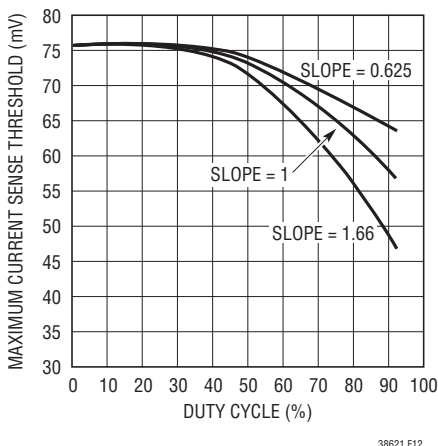
Figure 12. Effect of Slope Gain on the Peak \text{SENSE} Threshold
