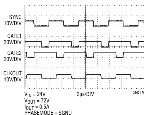
Figure 7: Synchronization of the LTC3862-1 to an External Clock Using the PLL
