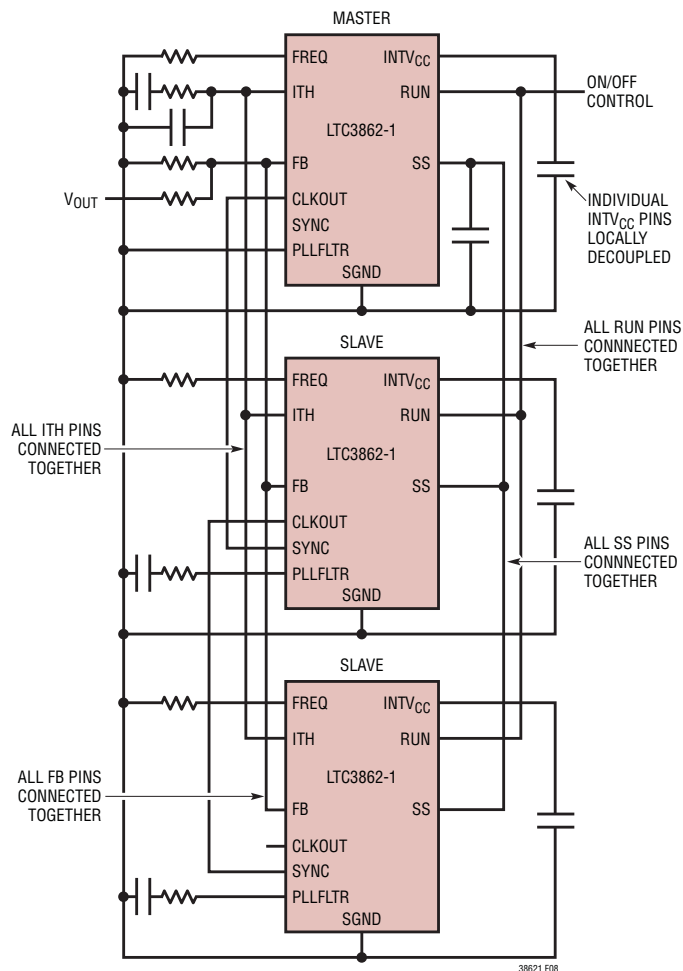
Figure 8. LTC3862-1 Error Amplifier Configuration for Multi-Phase Operation
