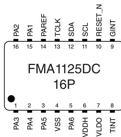
16-Pin SOP
