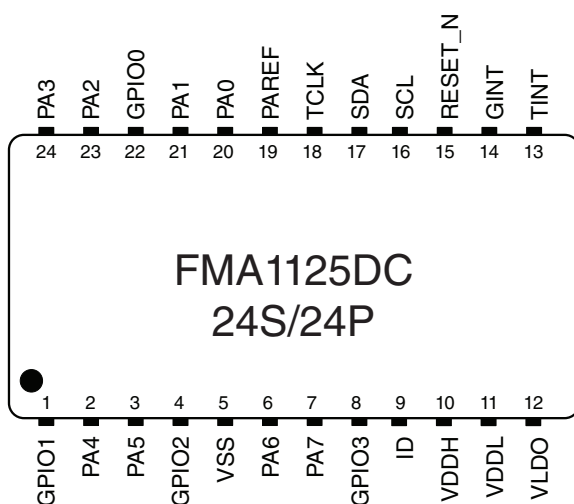
24-Pin SOP/SSOP
