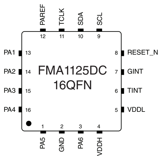
16-Pin QFN
