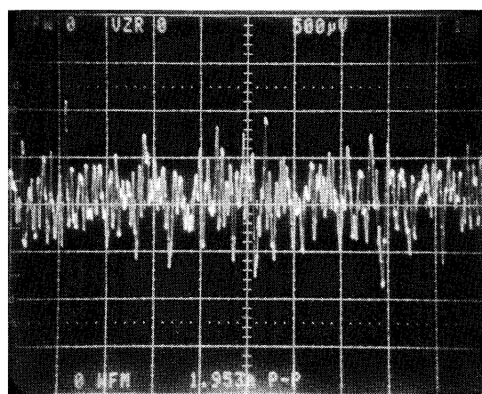
A_{\text{CL}} = 25,000\text{V/V} ; E_N = 0.08\mu\text{V}_{\text{P-P RTI}} Horizontal Scale = 1s/DIV; Vertical Scale = 0.02μV/DIV
