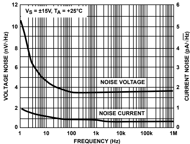
FIGURE 8. NOISE CHARACTERISTICS
