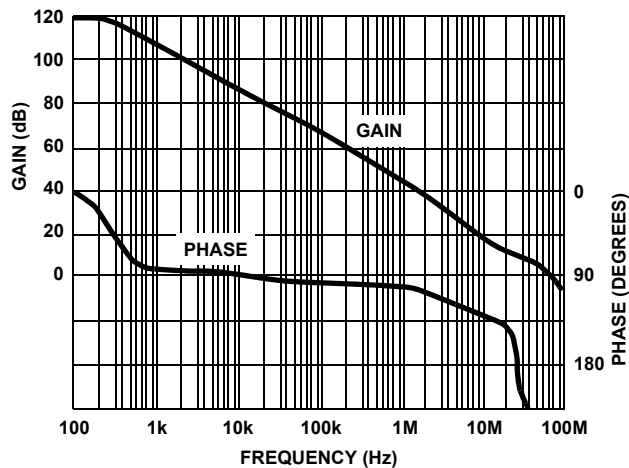
FIGURE 12. OPEN LOOP GAIN AND PHASE vs FREQUENCY
