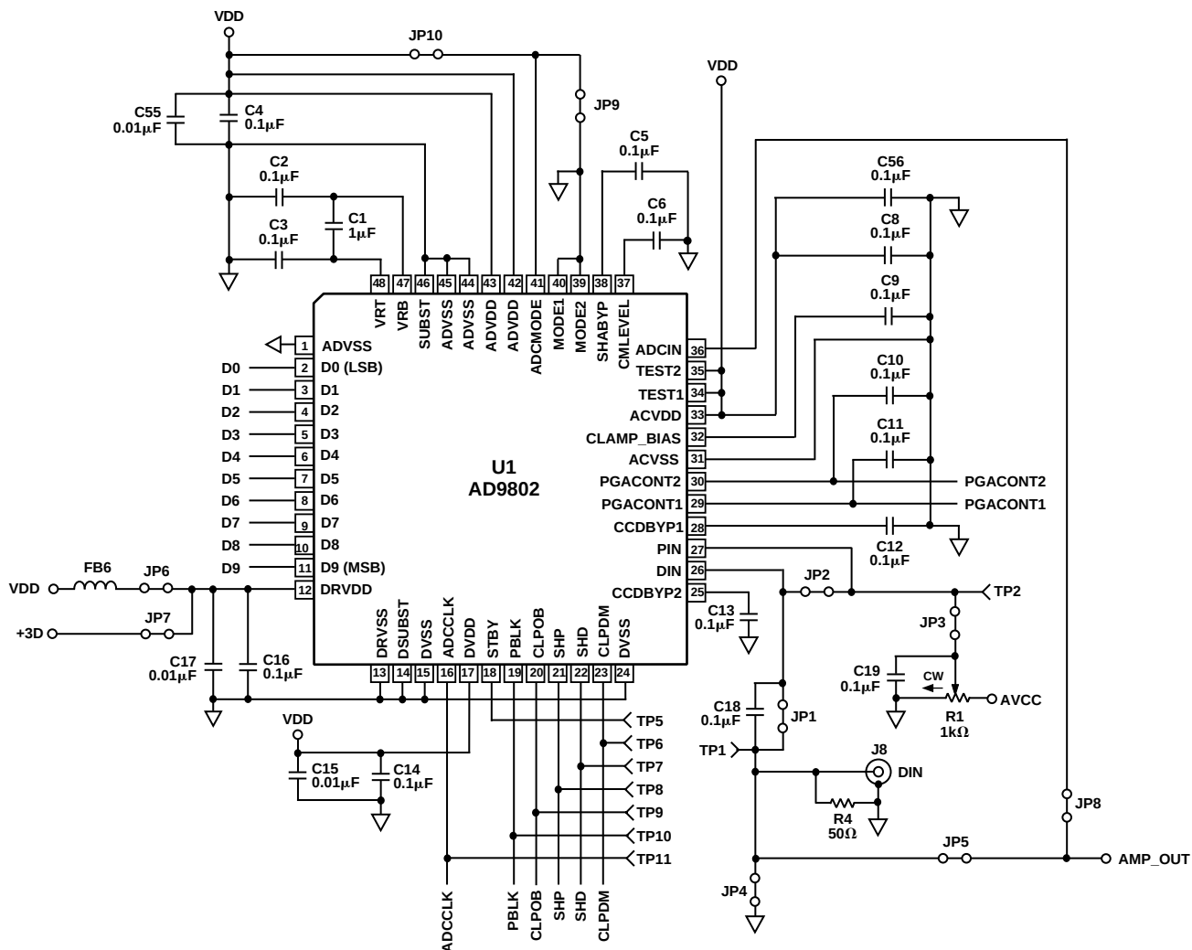
Figure 31. Evaluation Board
