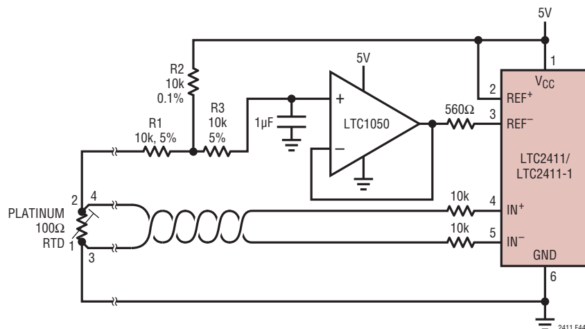
Figure 44. Remote Half Bridge Sensing with Noise Suppression on Reference
