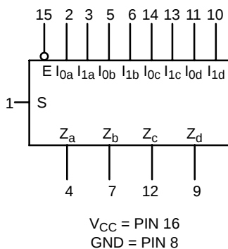
Figure 2. Logic Symbol
