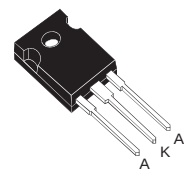
TO-247 STTH60P03SW
