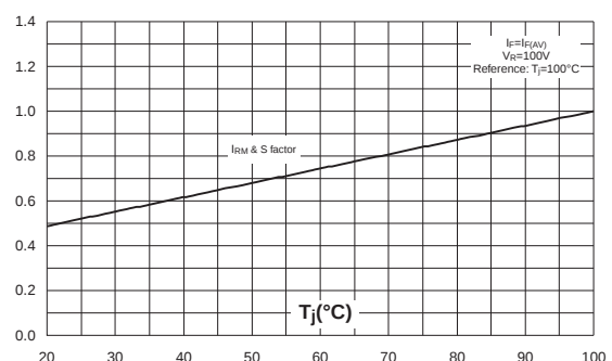
Figure 6. Relative variations of dynamic parameters versus junction temperature
